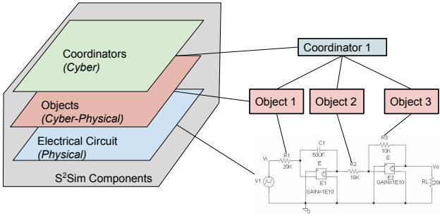
Fig. 2. CPS Layers of S 2 Sim.
