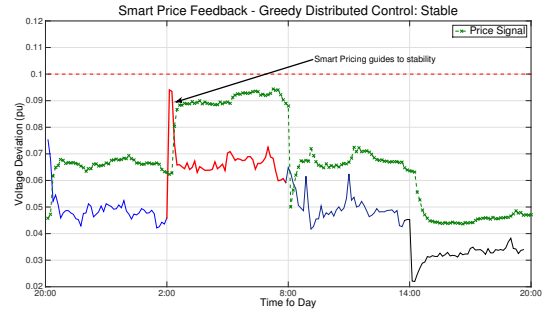
(b) Adaptive Pricing resulting in stable system behavior
