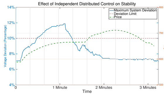
(b) Effect of Distributed Heterogeneous Control on system stability
