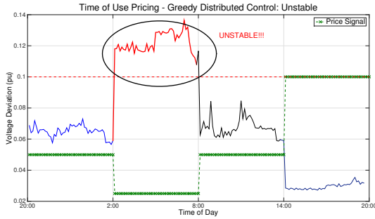
(a) Time of Use Pricing resulting in unstable system behavior
